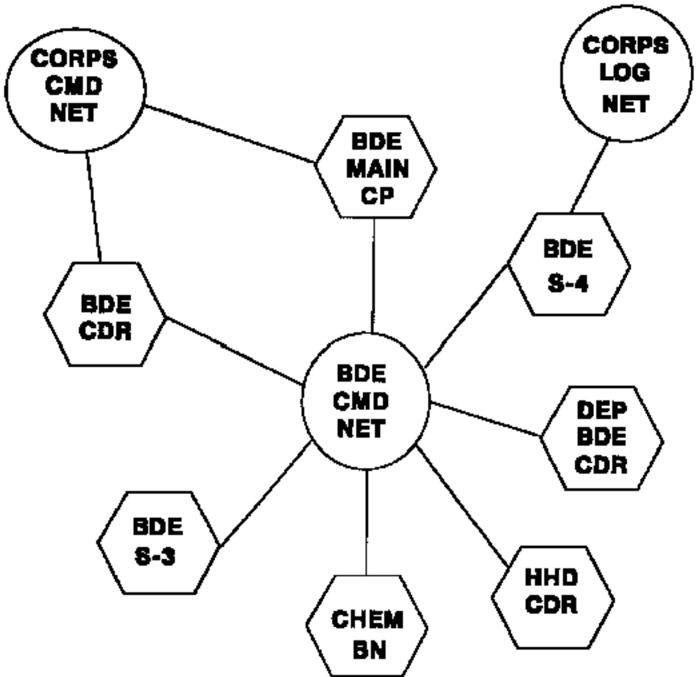
Figure 4-1. Radio net diagram (FM) for a chemical brigade HHD.
